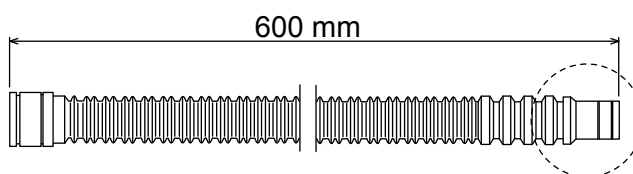
Drain hose
